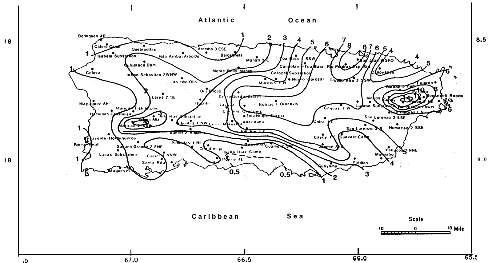
Figure 4-8. Hurricane Hugo rainfall (inches) for Puerto Rico.
