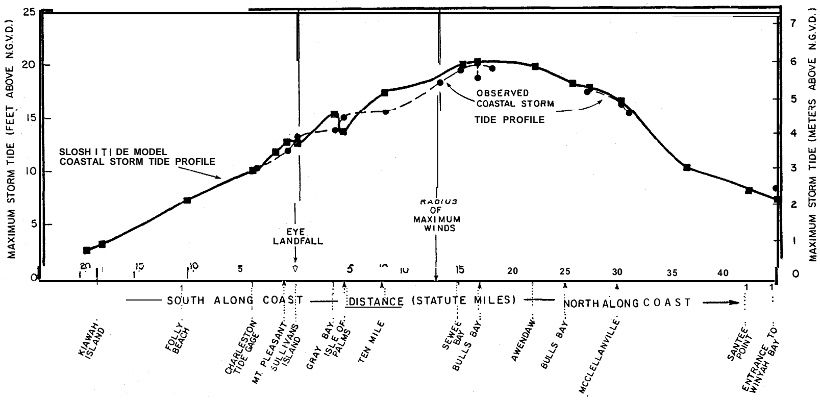
Figure 4-6. Distribution of storm tides along the South Carolina coast from Kiawah Island to Winah Bay. The solid line represents the preliminary SLOSH run of Fig. 4-5. The dashed line connects values of observed high storm tide. Values are given in feet above NGVD.
